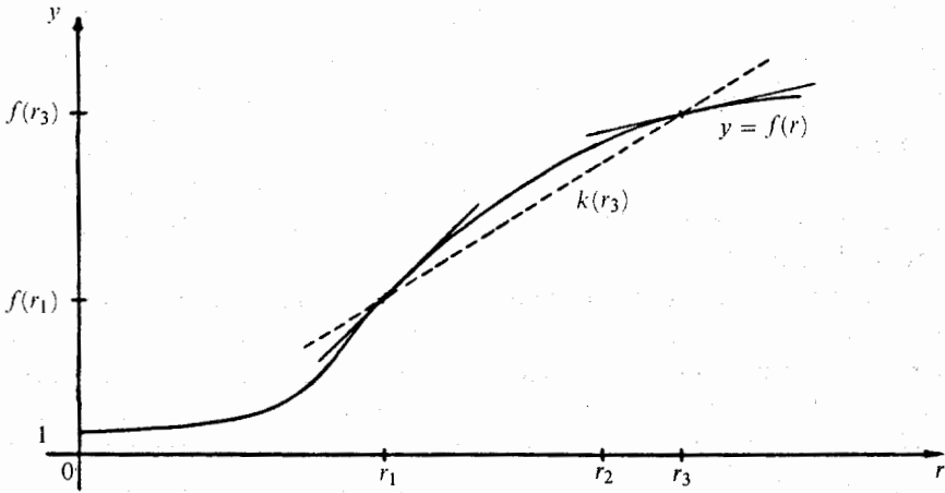
FIGURE 1. THE CONSTRUCTION OF THE FUNCTION f(r)
